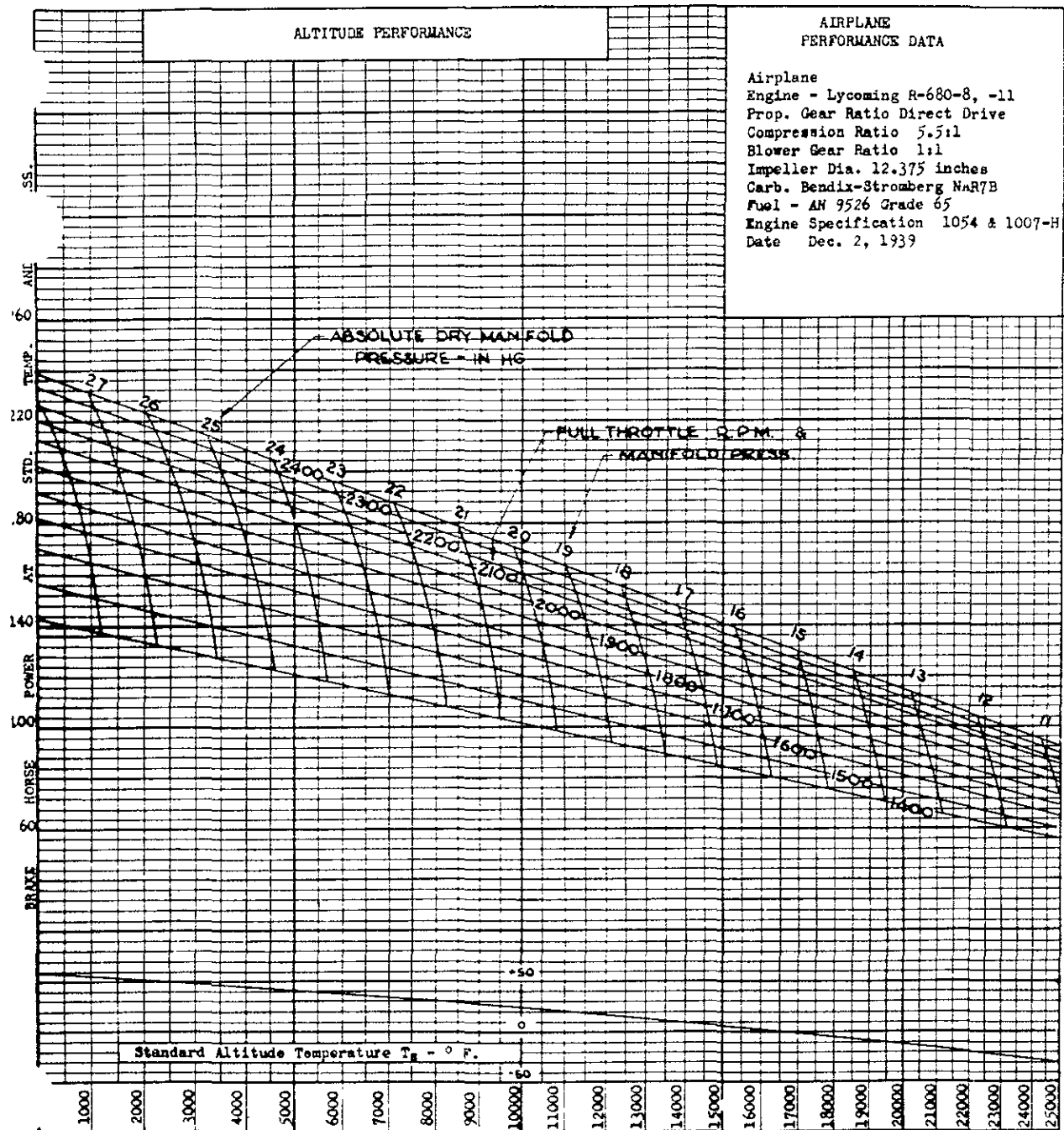
Figure 16 PRESSURE ALTITUDE IN FEET - 36 -
