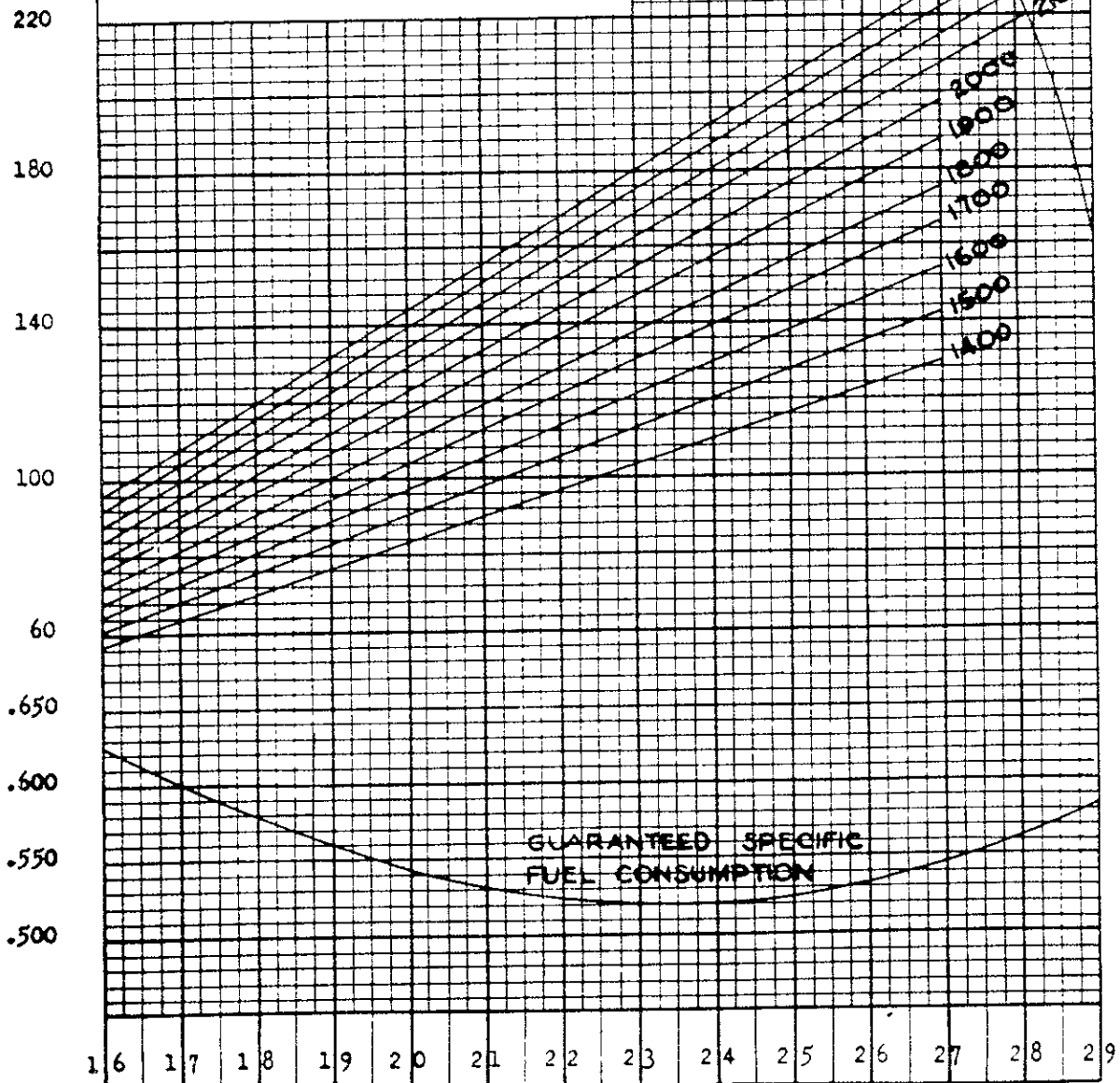
Figure 17 ABSOLUTE MANIFOLD PRESSURE, IN. HG.
